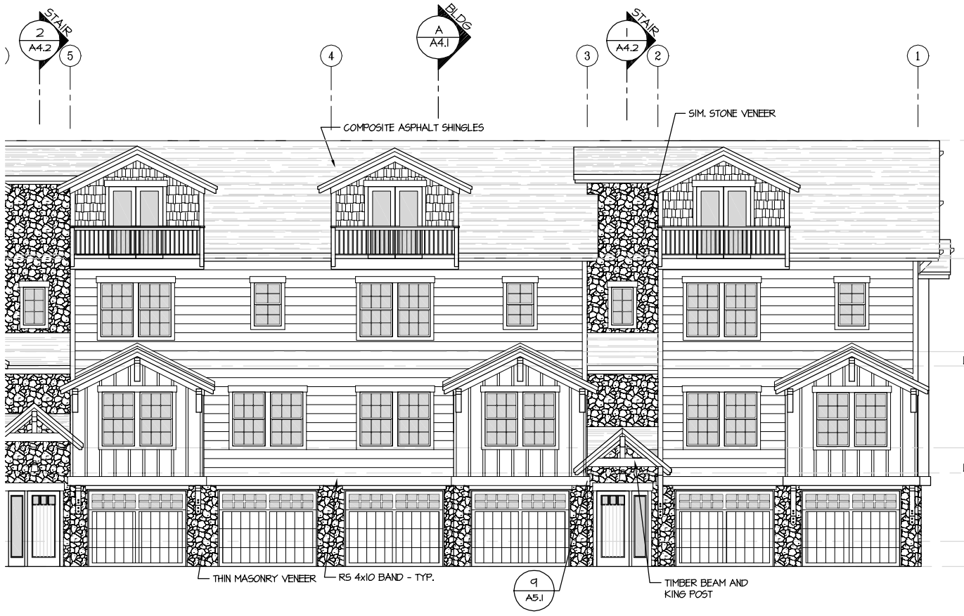
1 NORTH ELEVATION 1/8" = 1'-0"
