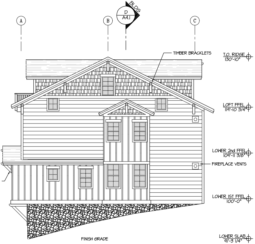
2 WEST ELEVATION 1/8" = 1'-0"
